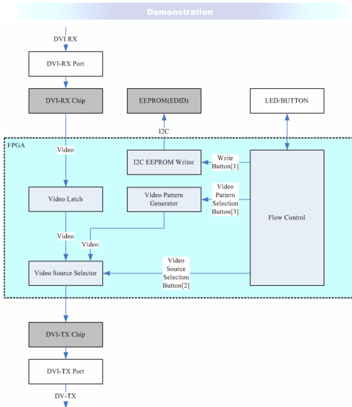
Figure 4.5.1 Block diagram
