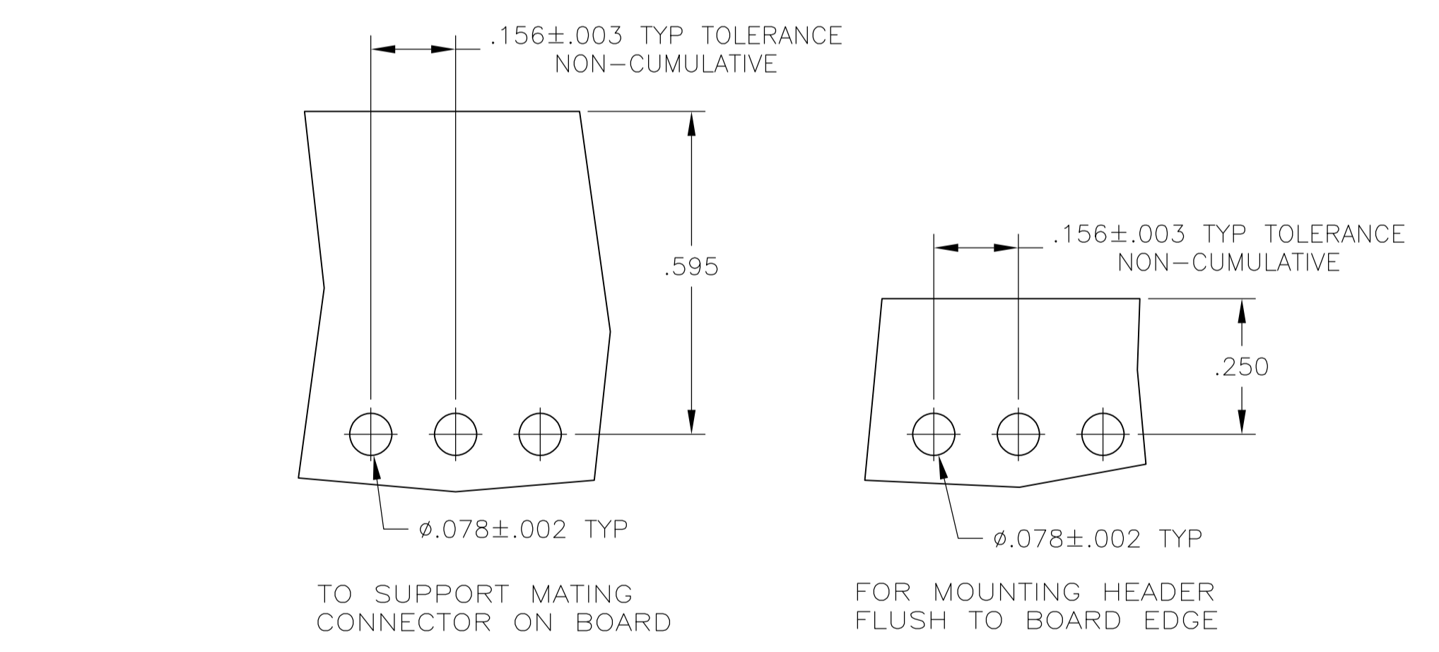
RECOMMENDED BOARD LAYOUTS
