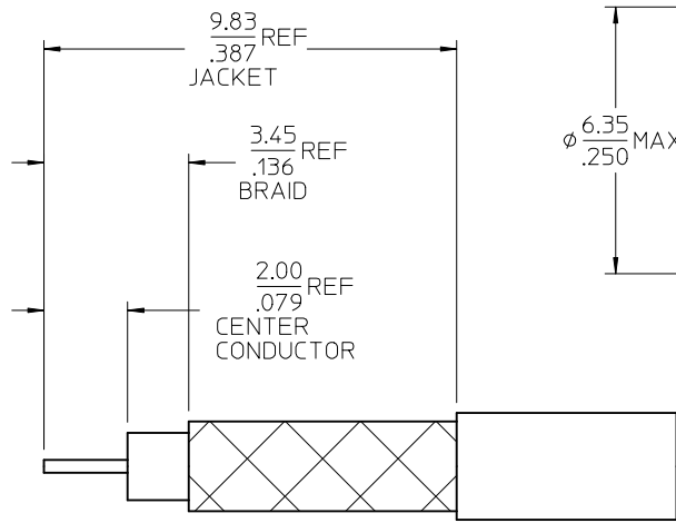
CABLE STRIP DIMENSIONS
